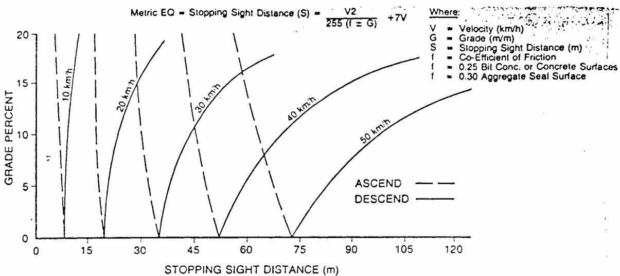
Figure 2 Stopping Sight Distance Calculation
